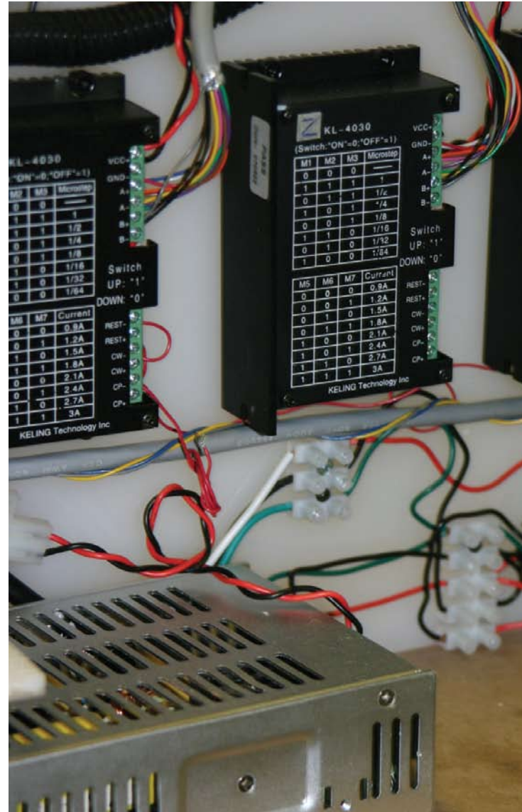
Wired KL4030 Stepper drivers & KL-201-24 Power Supply.
